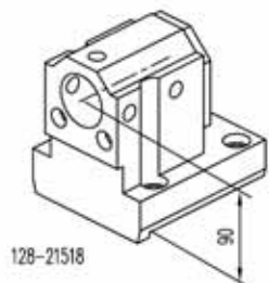
Combi toolholder for boring bar and insert drill
