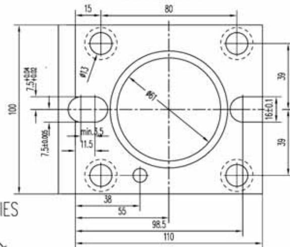
Drill socket
