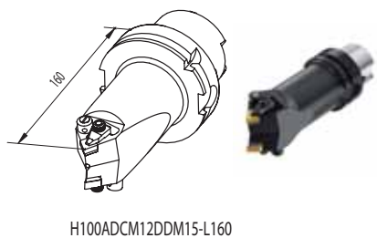
H100ADCM12DDM15-L160
