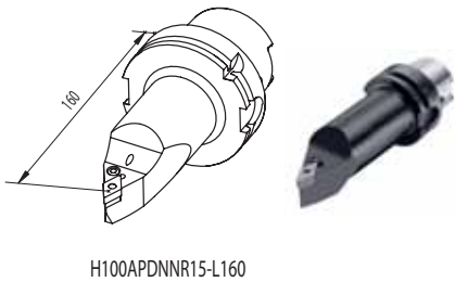
H100APDNNR15-L160
