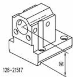
Toolholder for boring bar
