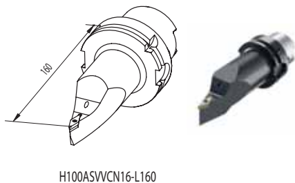
H100ASVVCN16-L160
